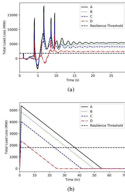
Fig. 7. Total load loss from Scenarios A, B, C, and D. (a) is dynamic response, (b) is steady-state response
