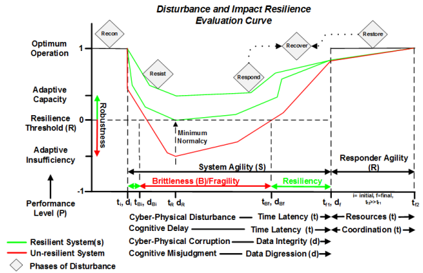
Fig. 2. Disturbance and Impact Resilience Evaluation Curve [29]
