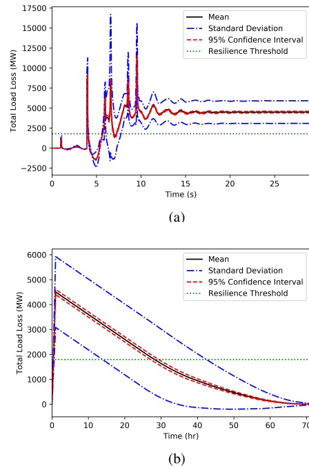
Fig. 8. Uncertainty Results with maximum DER penetration of 50% (a) dynamic response (b) steady state response
